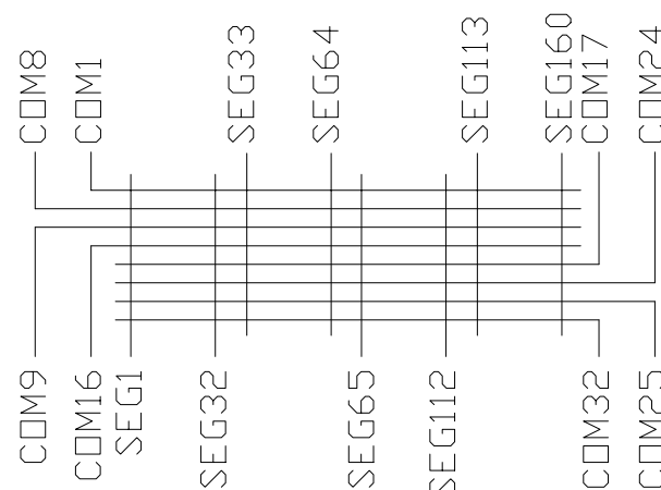
Wiring Details Scale=free
