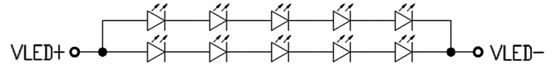
CIRCUIT DIAGRAM
