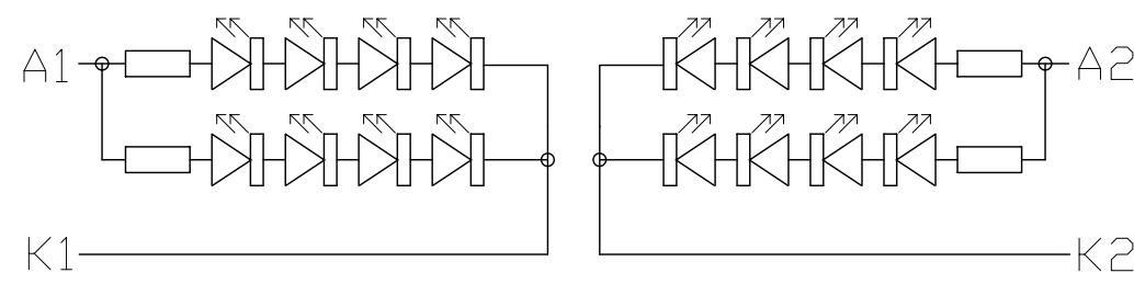
Backlight Circuit Details (No. of LED = 2x8=16pcs) Scale=free
