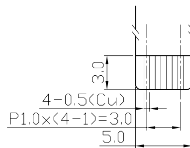
Touch Panel FFC Terminals Details (Conductor Side) Scale=3/1
