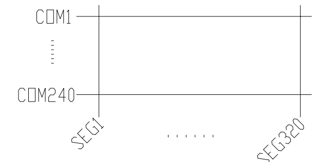
Wiring Details(Top View) Scale=Free
