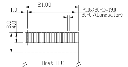
Conductor Side Details Scale=2/1
