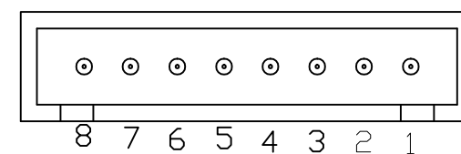
K1(scale 4:1): 8Pin pitch=2.50mm Part No: SYUIN 8824-08
