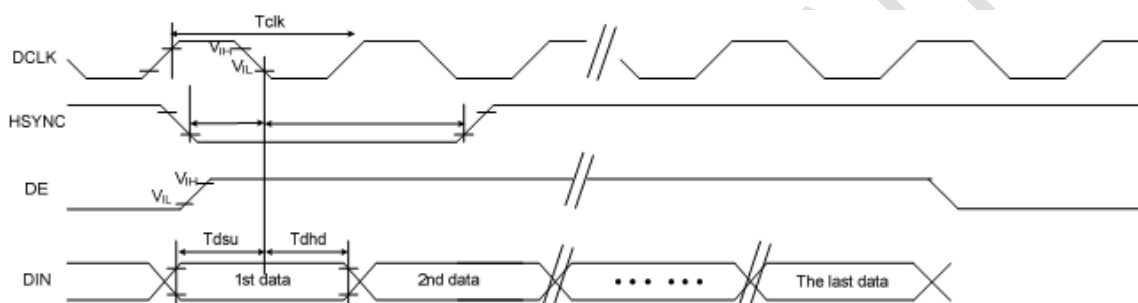
Figure 5.2.1.2 SYNC-DE Mode
