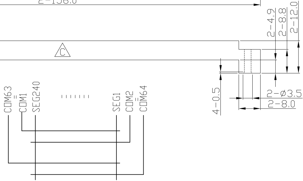
Wiring Details(Top View) Scale=free
