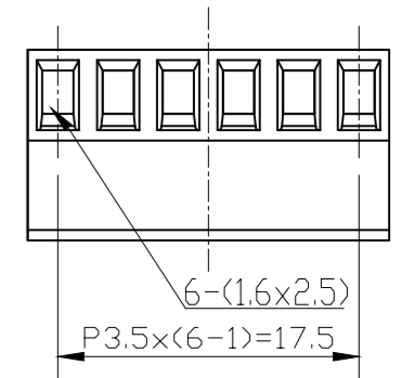
K1 Details Scale=2/1
