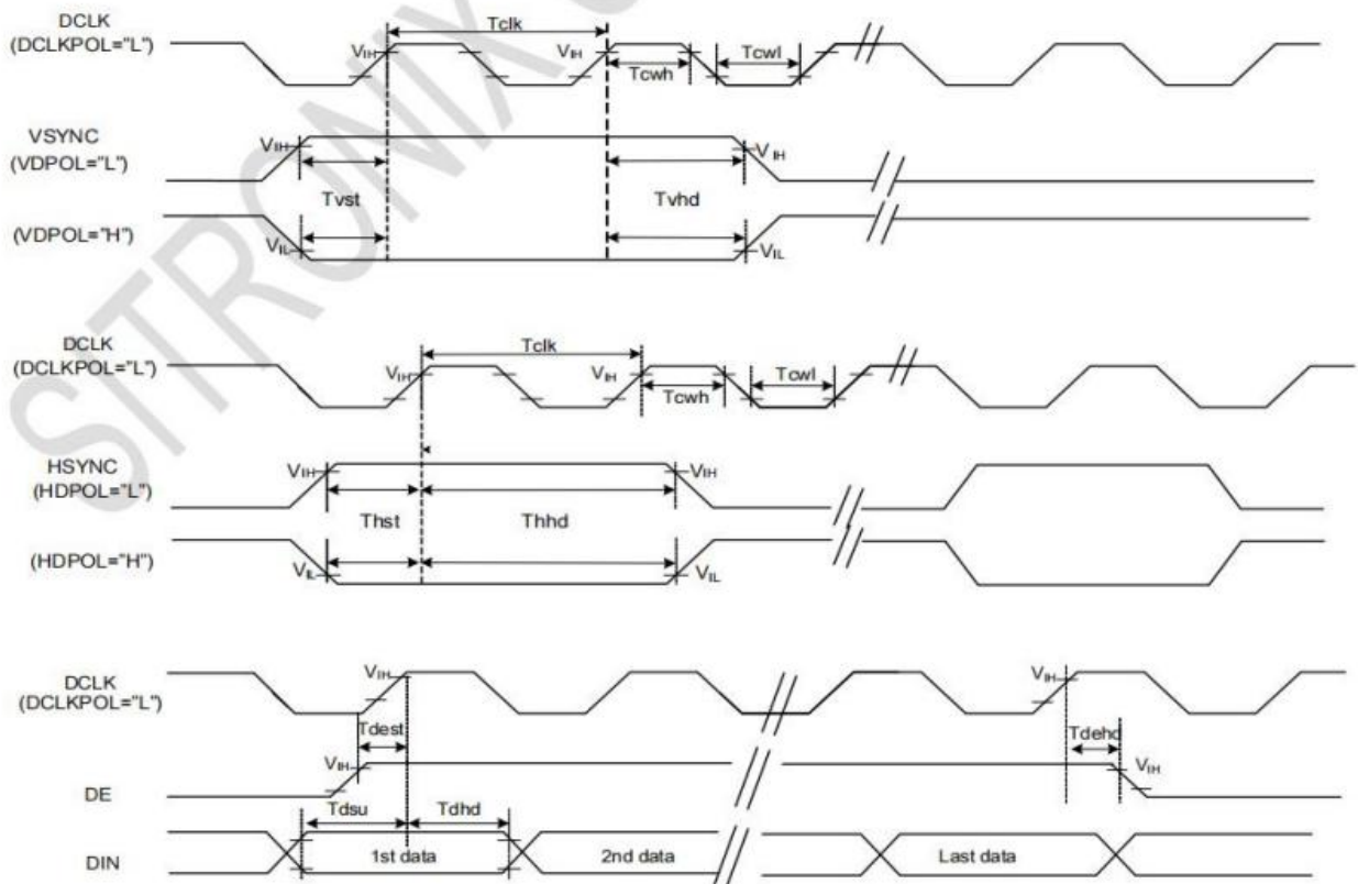
Timing Diagram
