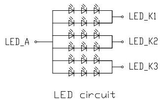
LED circuit
